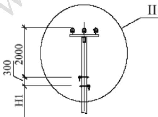
Starpbalsts S20.I-HT-04Ps
